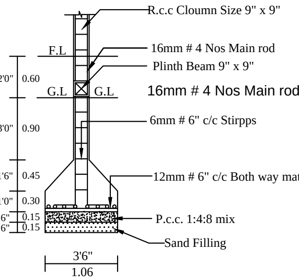
COLUMN DETIAL
