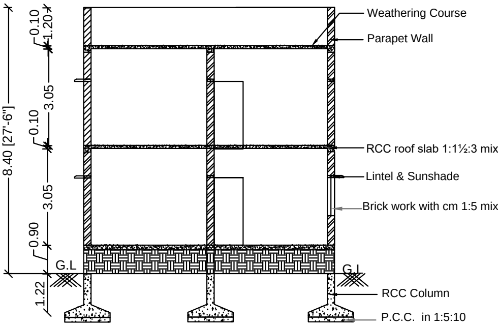
SECTION - "AB"
