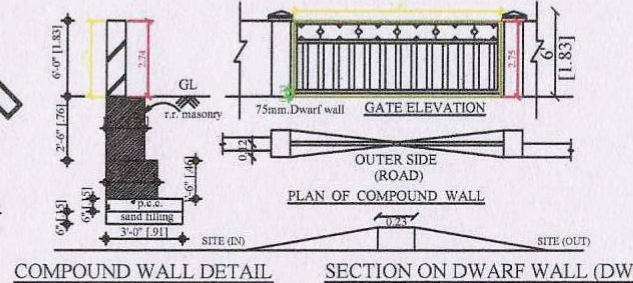
COMPOUND WALL DETAIL
