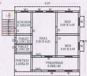
EXISTING GROUND FLOOR PLAN
