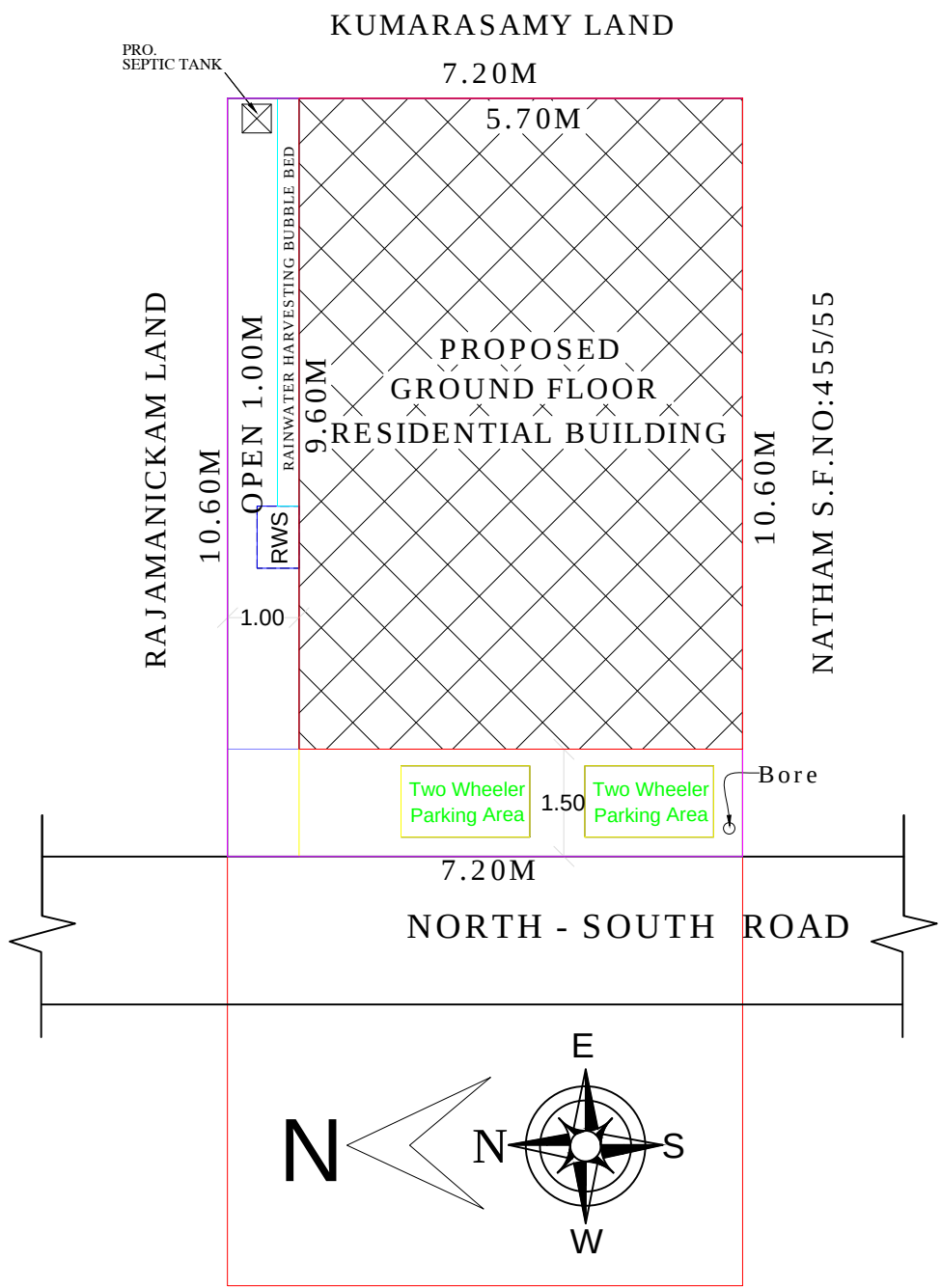
SITE PLAN
