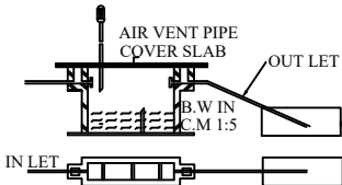
DETAILS OF SEPTIC TANK & D-TRENCE
