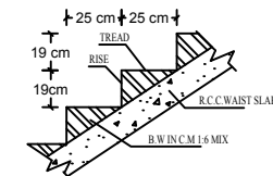
SECTION OF STAIRCASE BORE WELL DETAIL
