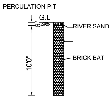
PERCOLATION PIT
