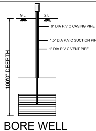
BORE WELL
