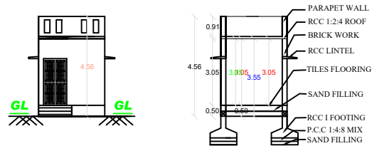
FRONT ELEVATION
