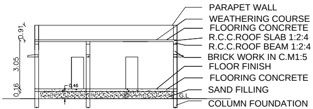
SECTION- SS
