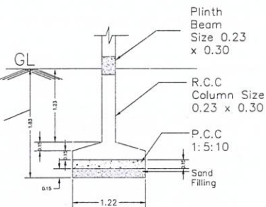
FOUNDATION DETAILS
