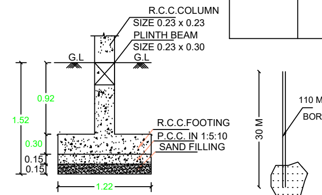
FOUNDATION DETAIL
