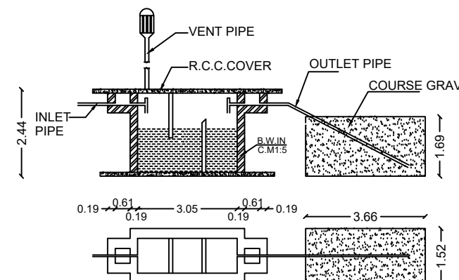
SEPTIC TANK & DISPERSION TRENCH DETAILS
