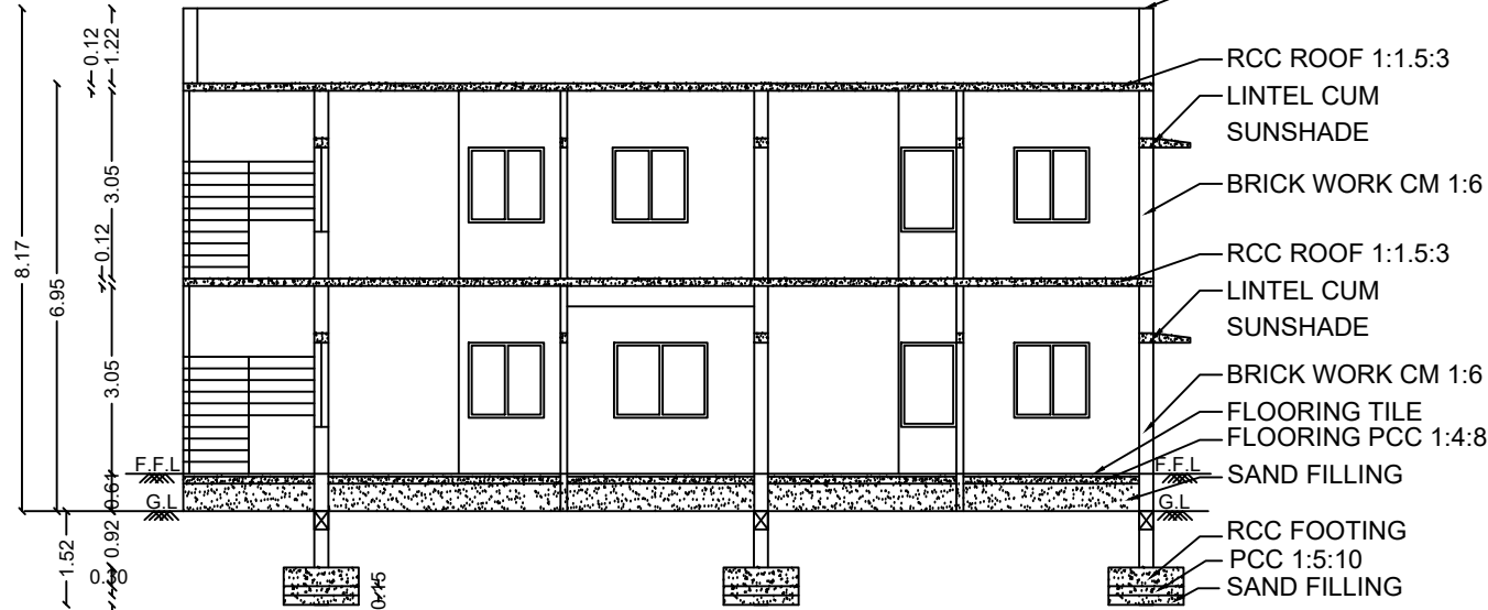
SECTION-AA
