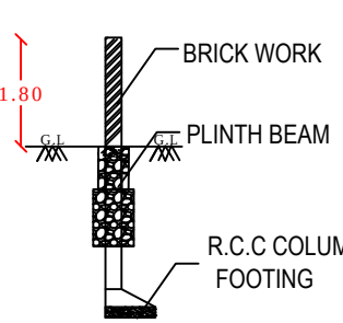
SECTION
