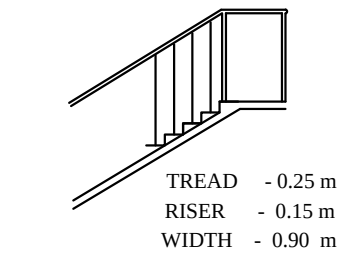
STAIRCASE DETAILS
