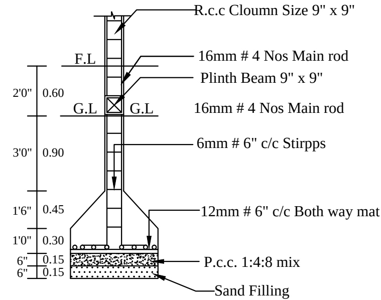
COLUMN DETIAL
