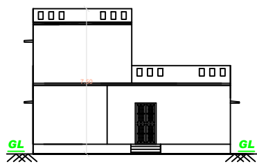
FRONT ELEVATION
