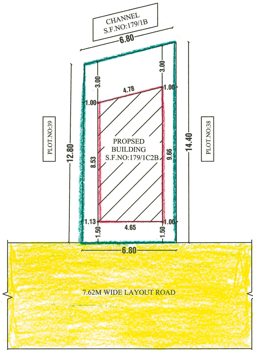
SITE PLAN
