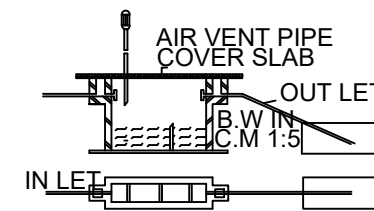
DETAILS OF SEPTIC TANK & D-TRENCE
