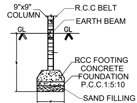
FOUNDATION DETAILS
