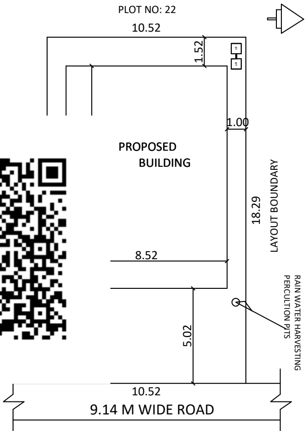
SITE PLAN
