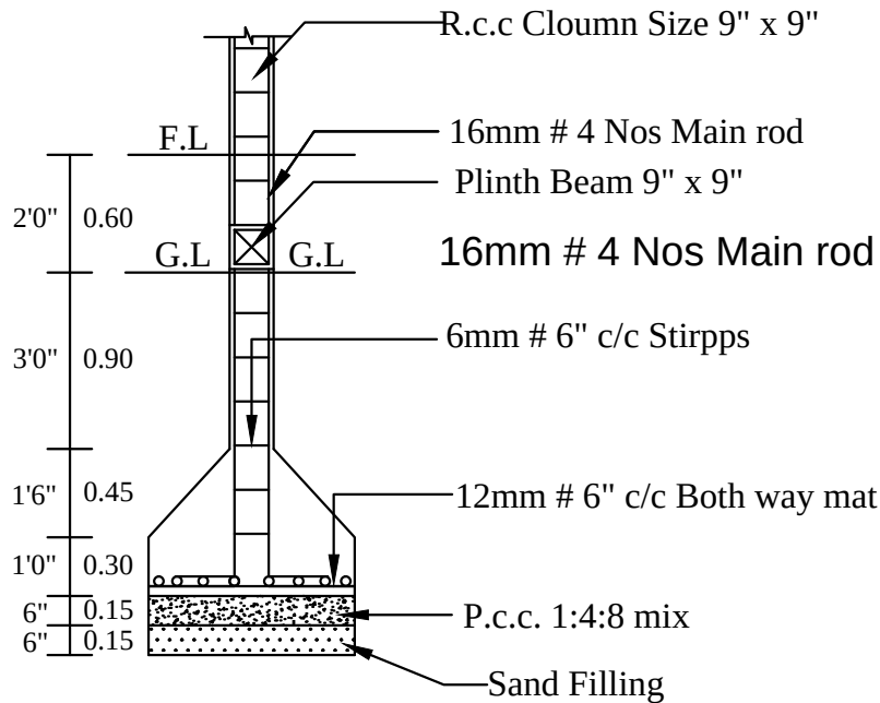
COLUMN DETAILS
