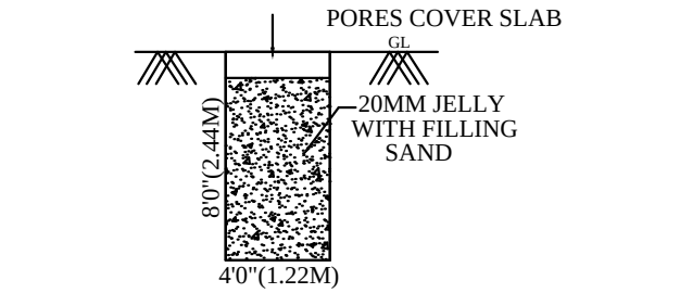
RAIN WATER HARVESTING UNIT
