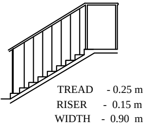
STAIRCASE DETAILS
