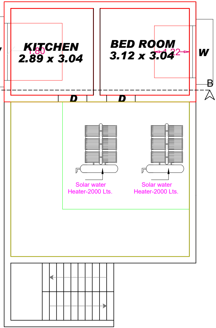
FIRST FLOOR PLAN & OPEN TERRACE PLAN
