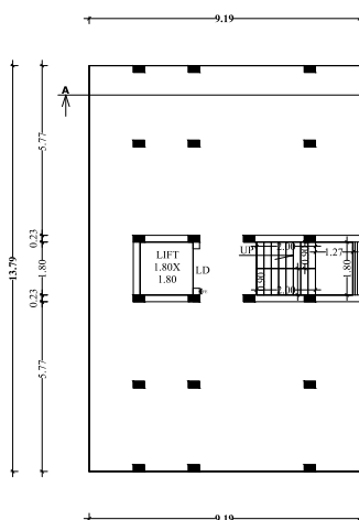
STILT FLOOR PLAN
