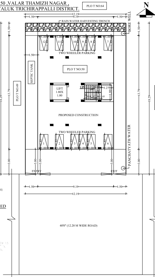
SITE PLAN
