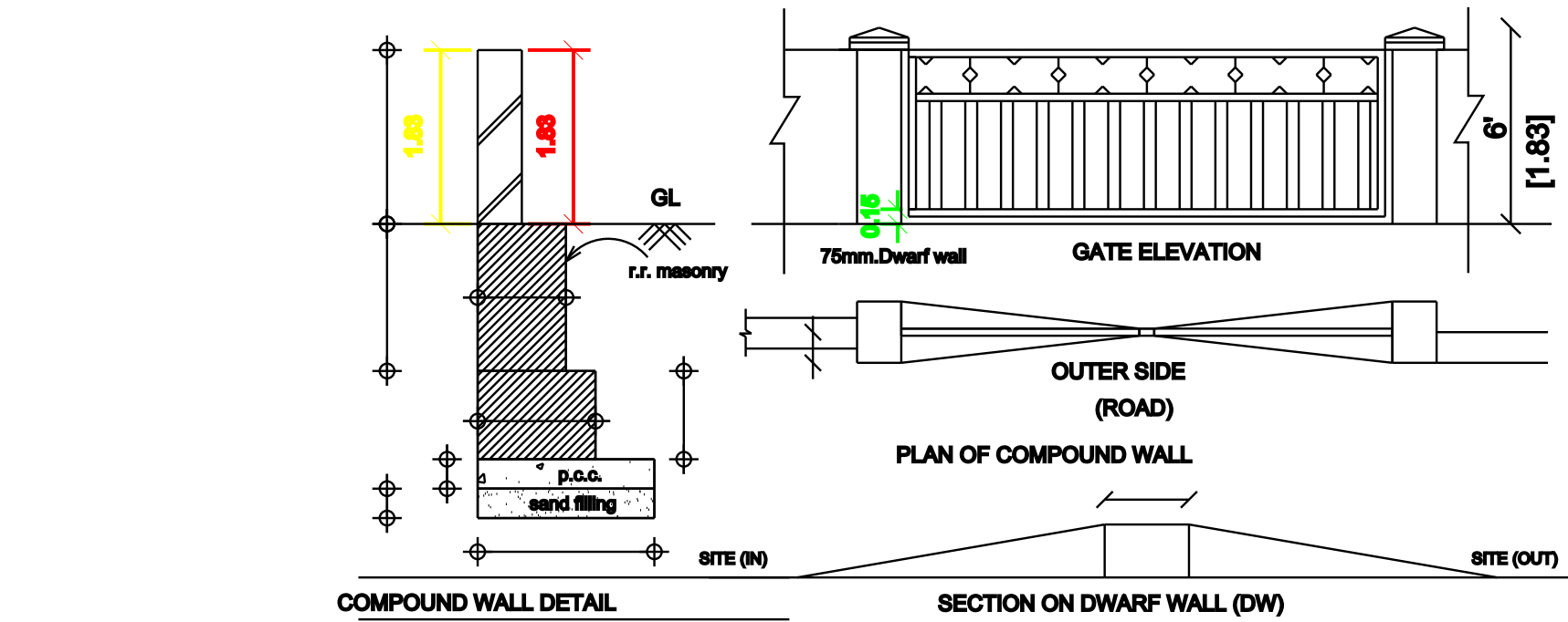
COMPOUND WALL DETAIL
