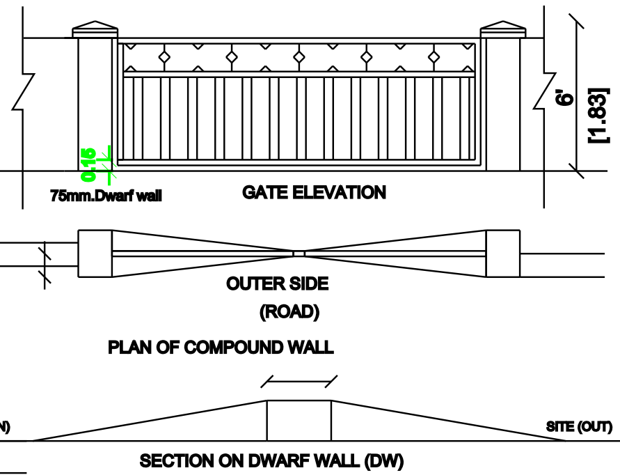
SECTION ON DWARF WALL (DW)
