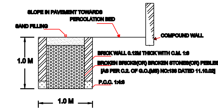
SECTION OF RAIN WATER PERCOLATION BED
