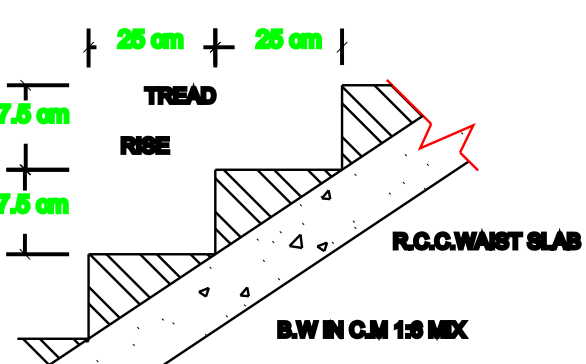
SECTION OF STAIRCASE
