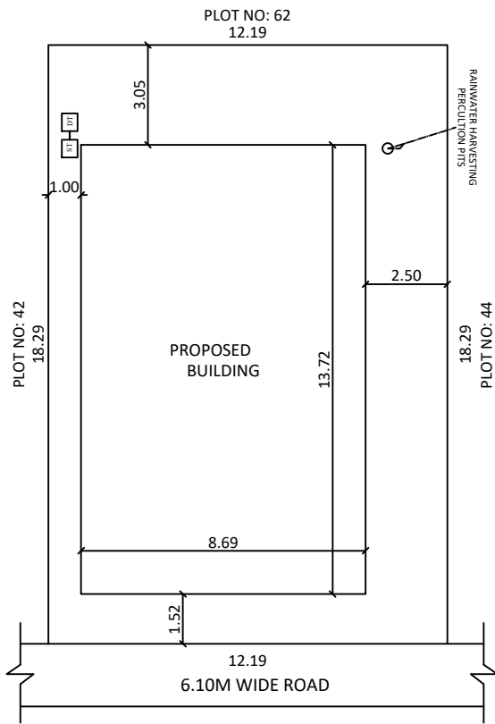
SITE PLAN
