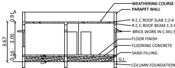
SECTION ON GG
