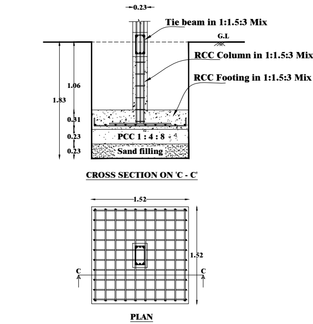
COLOUMN FOUNDATION DETAILS
