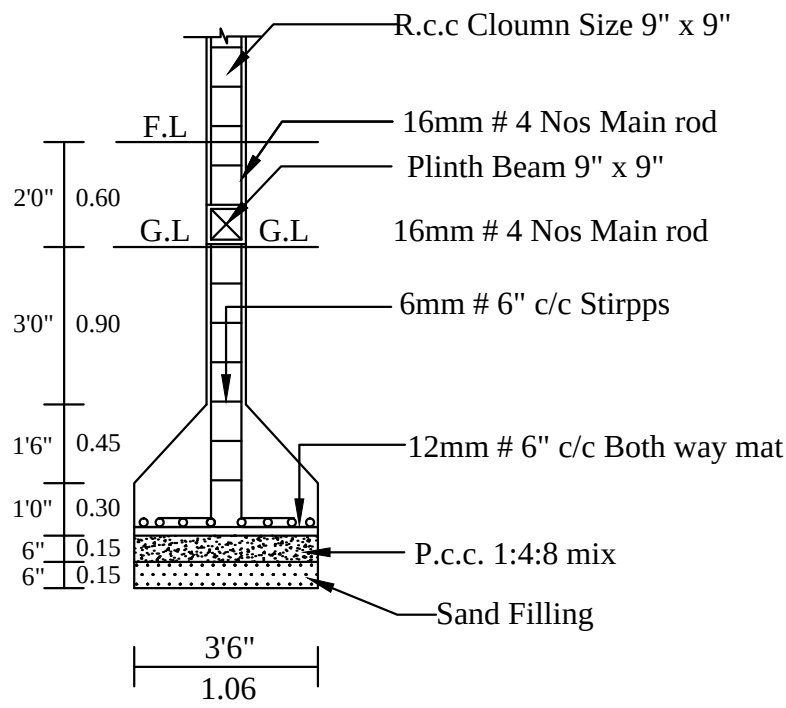
COLUMN DETIAL
