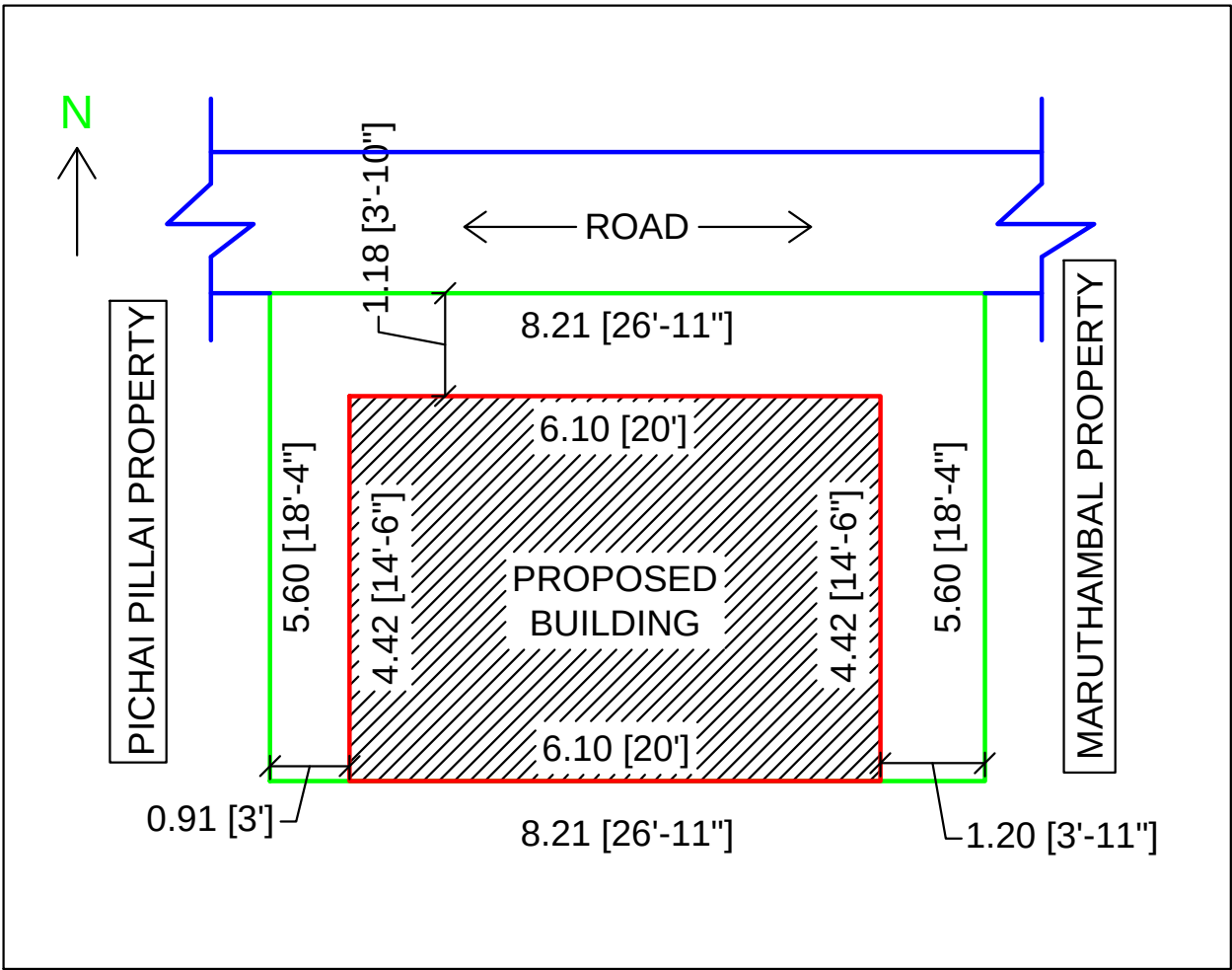
SITE PLAN (1:100)
