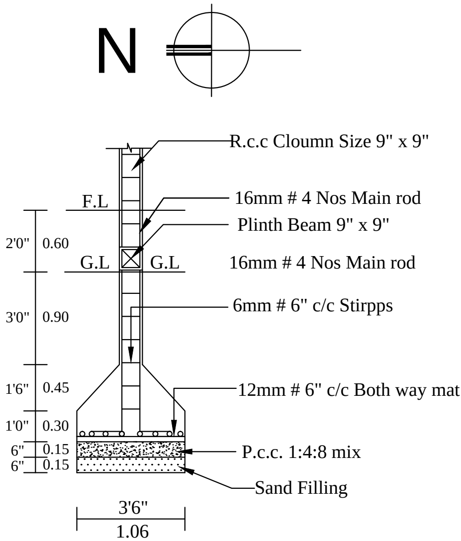
COLUMN DETIALS
