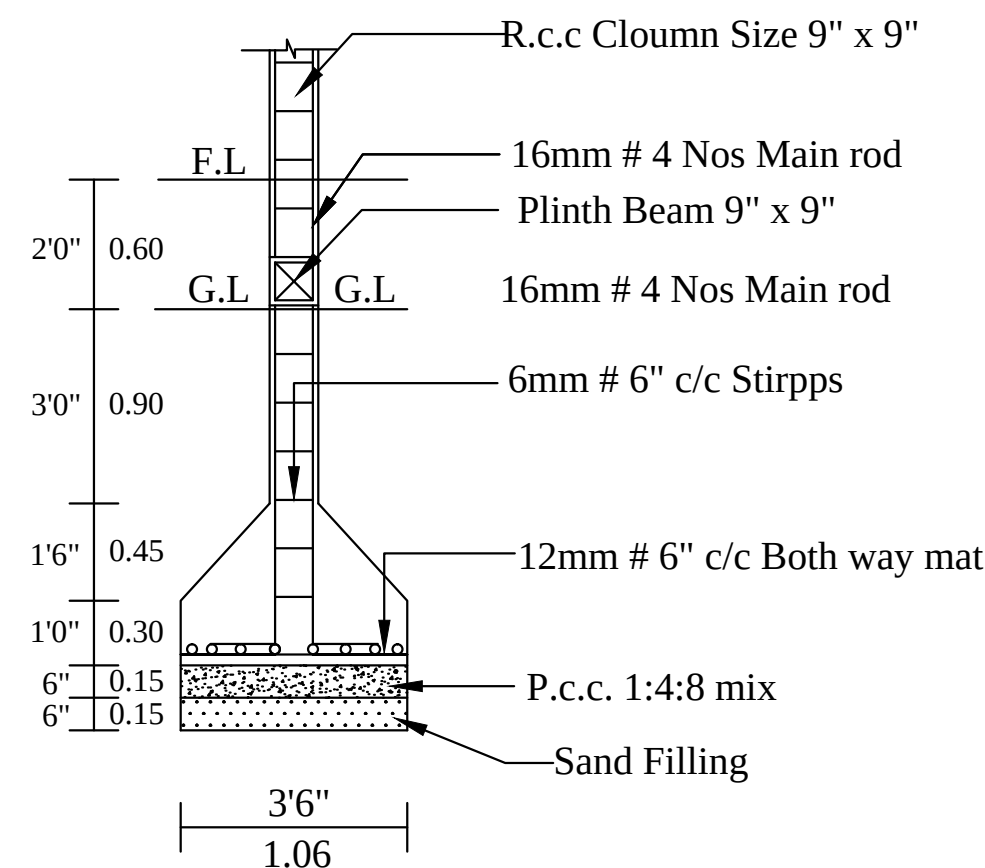
COLUMN DETAILS
