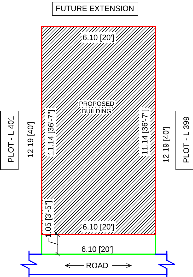
SITE PLAN (1:100)
