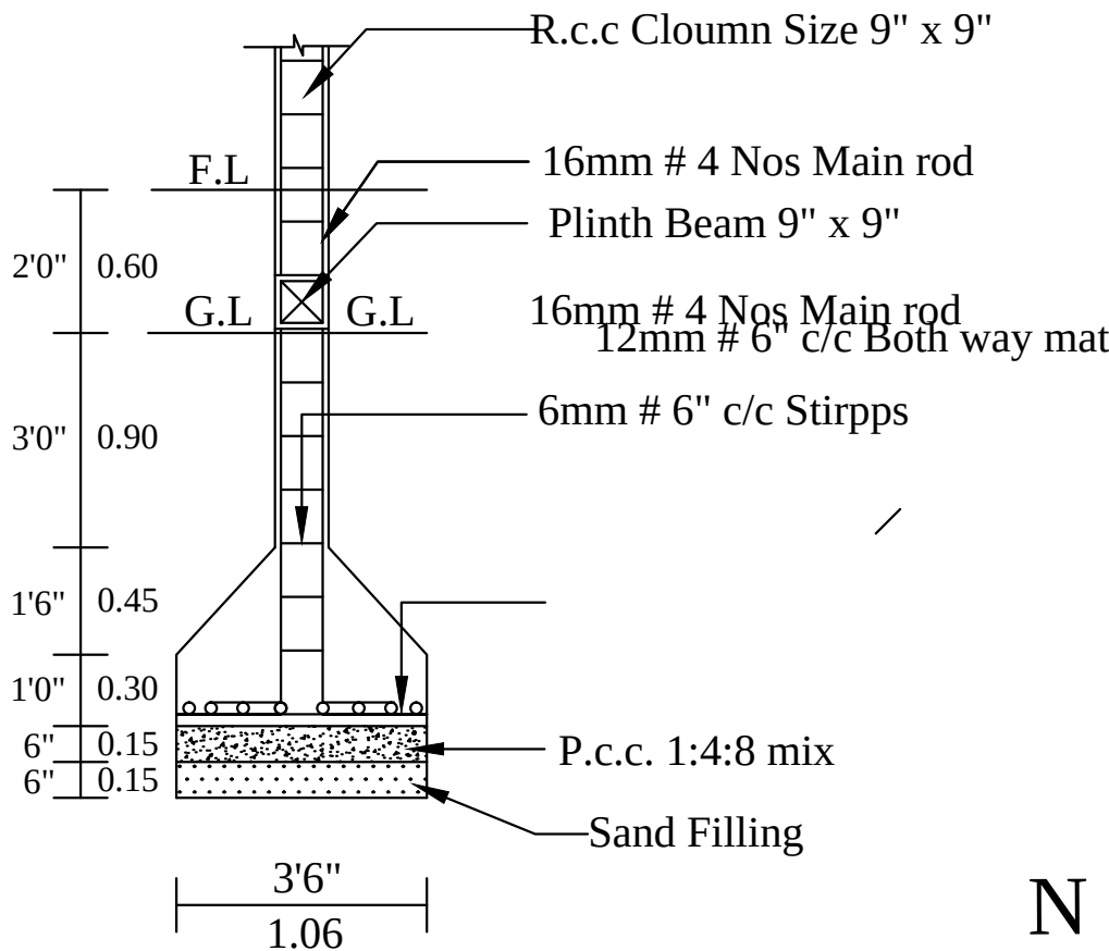
COLUMN DETIAL
