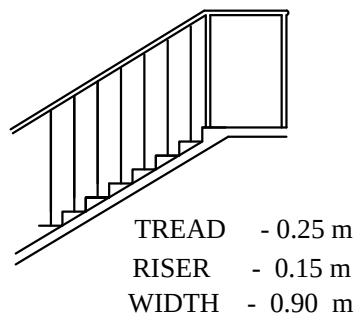
STAIRCASE DETAILS
