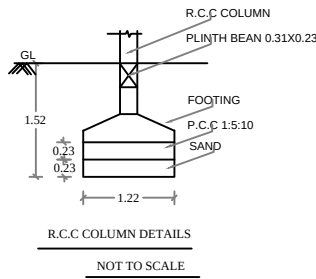
R.C.C. COLUMN DETAILS
