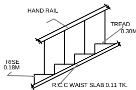
STAIR CASE DETAILS
