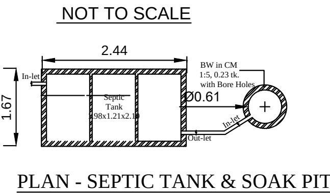
PLAN - SEPTIC TANK & SOAK PIT
