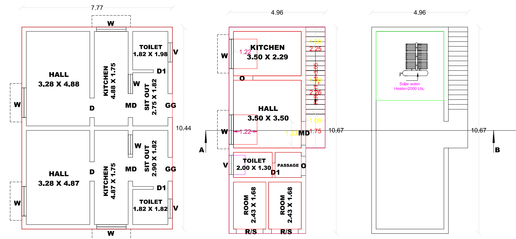
EXISTING GF PLAN
