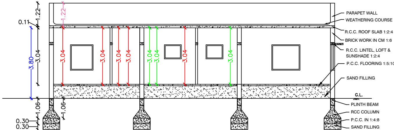
SECTION AA
