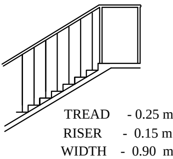
STAIRCASE DETAILS
