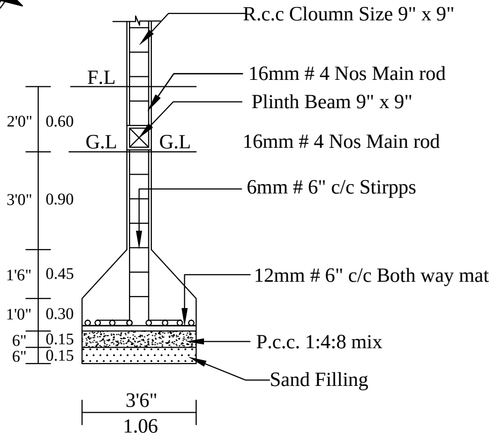
COLUMN DETIAL
