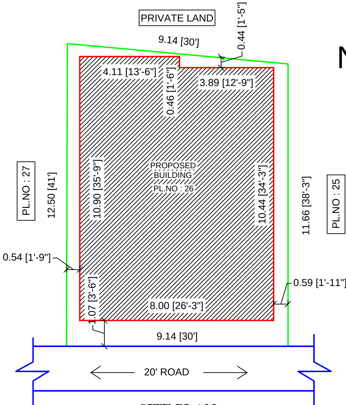
SITE PLAN
