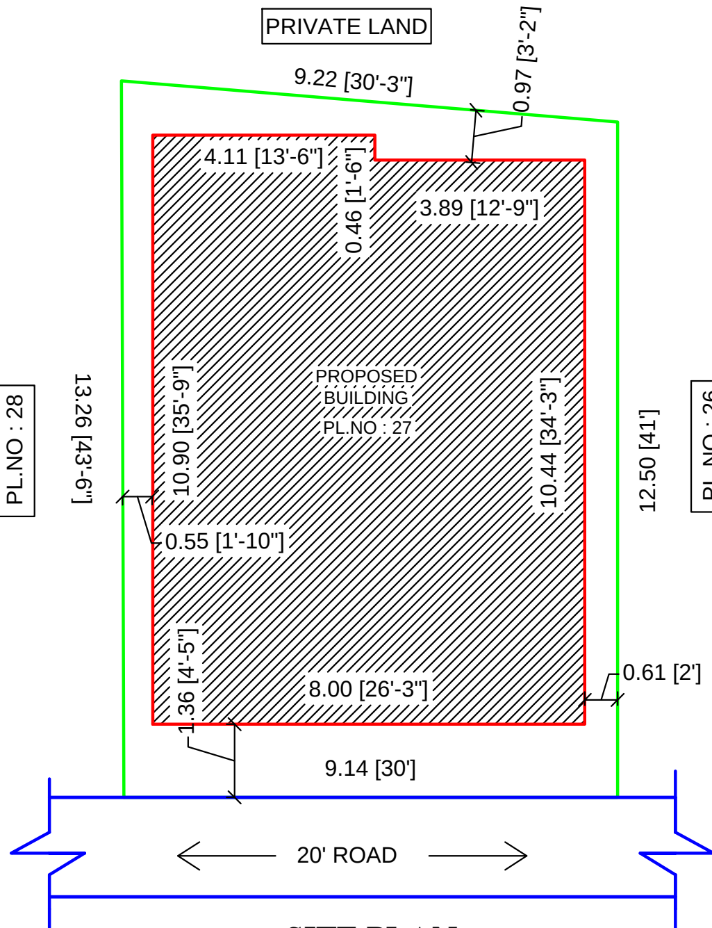
SITE PLAN (1:100)
