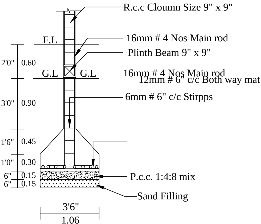
COLUMN DETIAL
