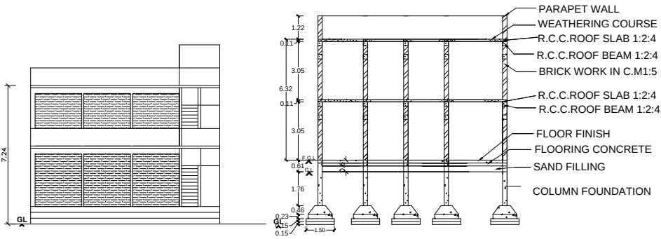
SECTION- SS
