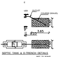
SEPTIC TANK & D-TRENCH DETAILS (NOT TO SCALE)
