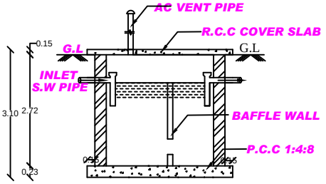
SAEPTIC TANK DETAILS
