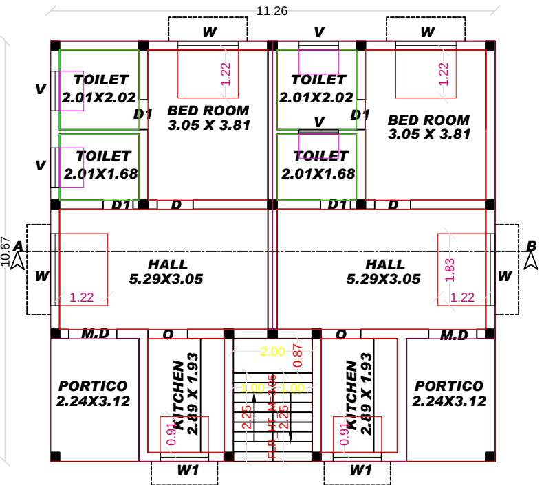
PRO.GROUND FLOOR PLAN (SOUTH FACING)
