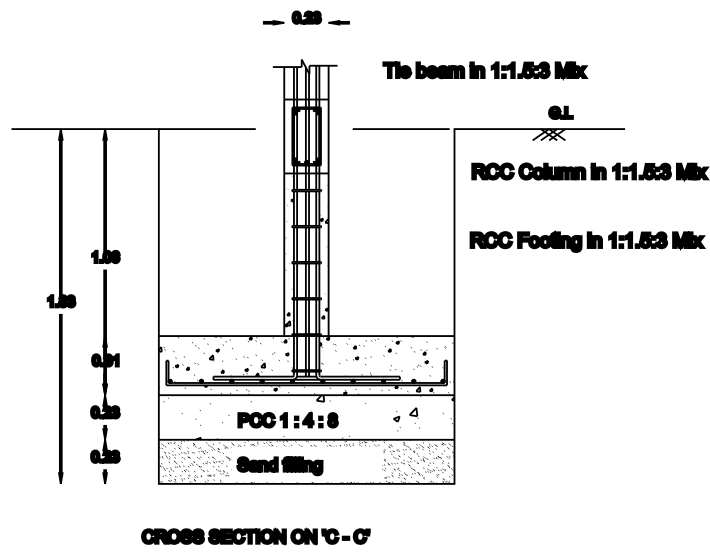
COLOUMN FOUNDATION DETAILS
