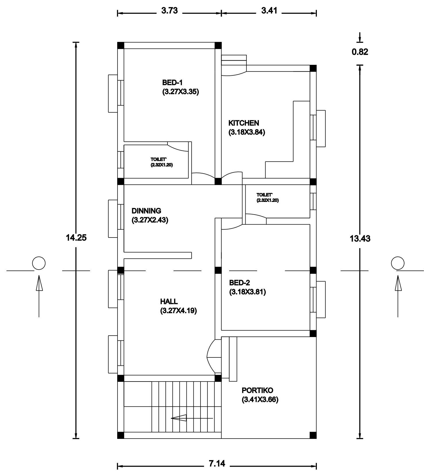
PLAN
