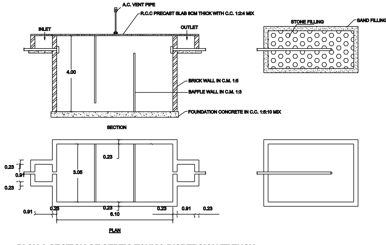
PLAN & SECTION OF SEPTIC TANK & DISPERSION TRENCH
