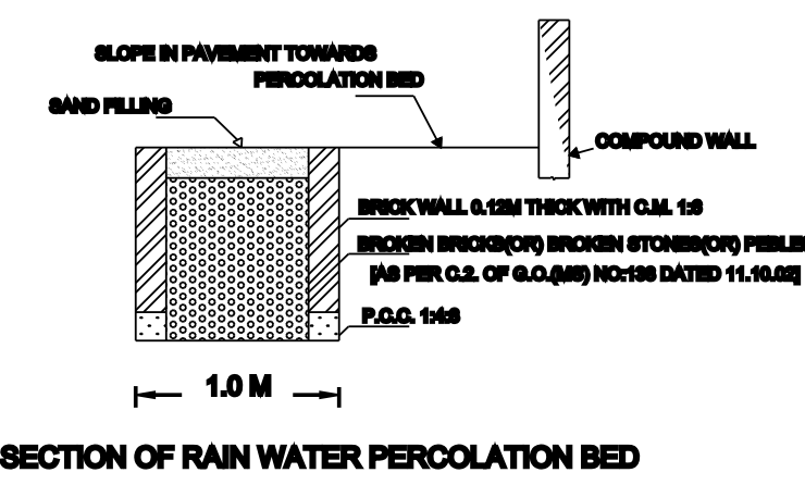
SECTION OF RAIN WATER PERCOLATION BED
