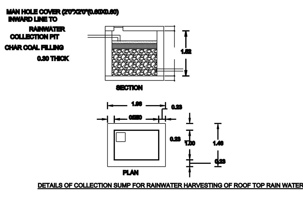
DETAILS OF COLLECTION PUMP FOR RAINWATER HARVESTING OF ROOF TOP RAIN WATER
