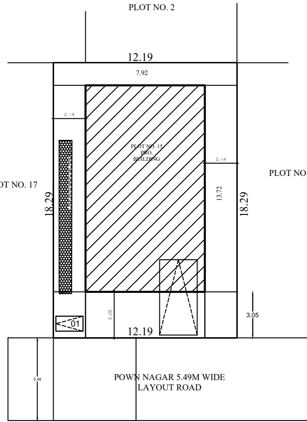
KEY PLAN
