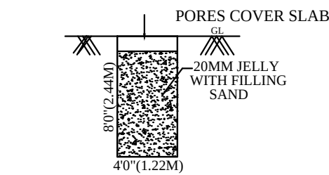
RAIN WATER HARVESTING UNIT
