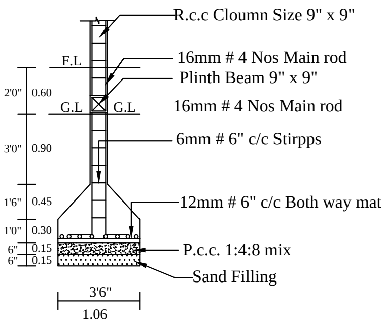
COLUMN DETIAL
