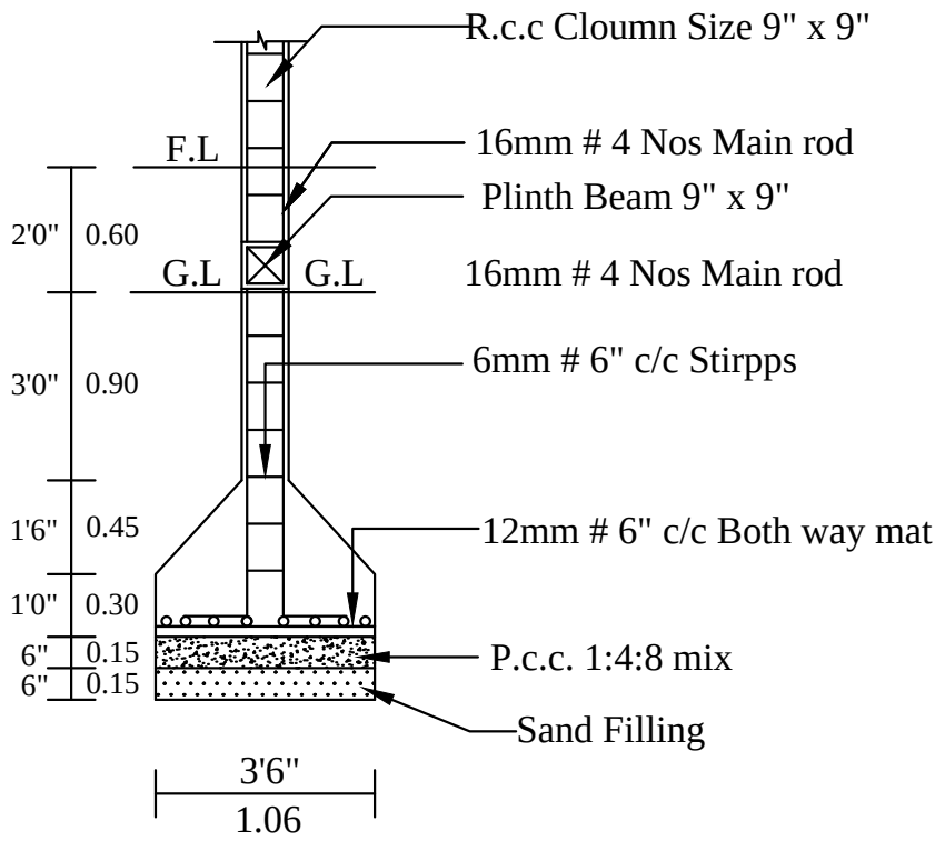
COLUMN DETIAL
