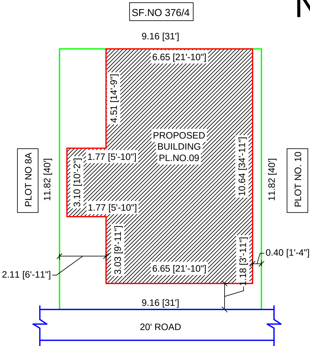
SITE PLAN (1:100)
