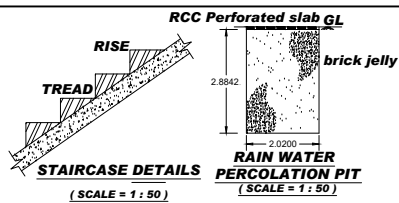
STAIRCASE DETAILS (SCALE = 1:50)
