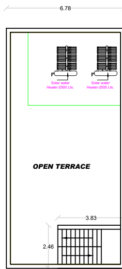
OPEN TERRACE PLAN
