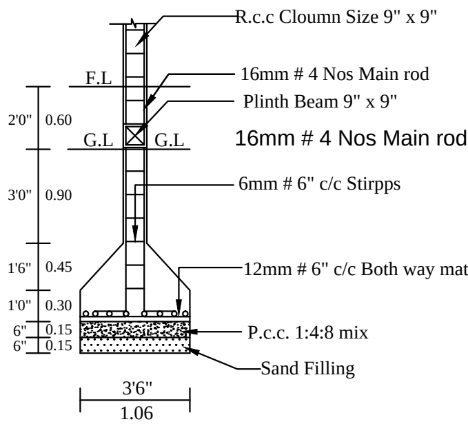
COLUMN DETIAL
