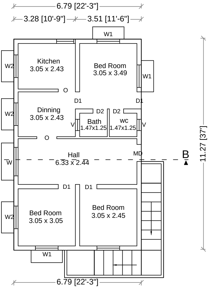
EXG & PRO. FIRST FLOOR PLAN
