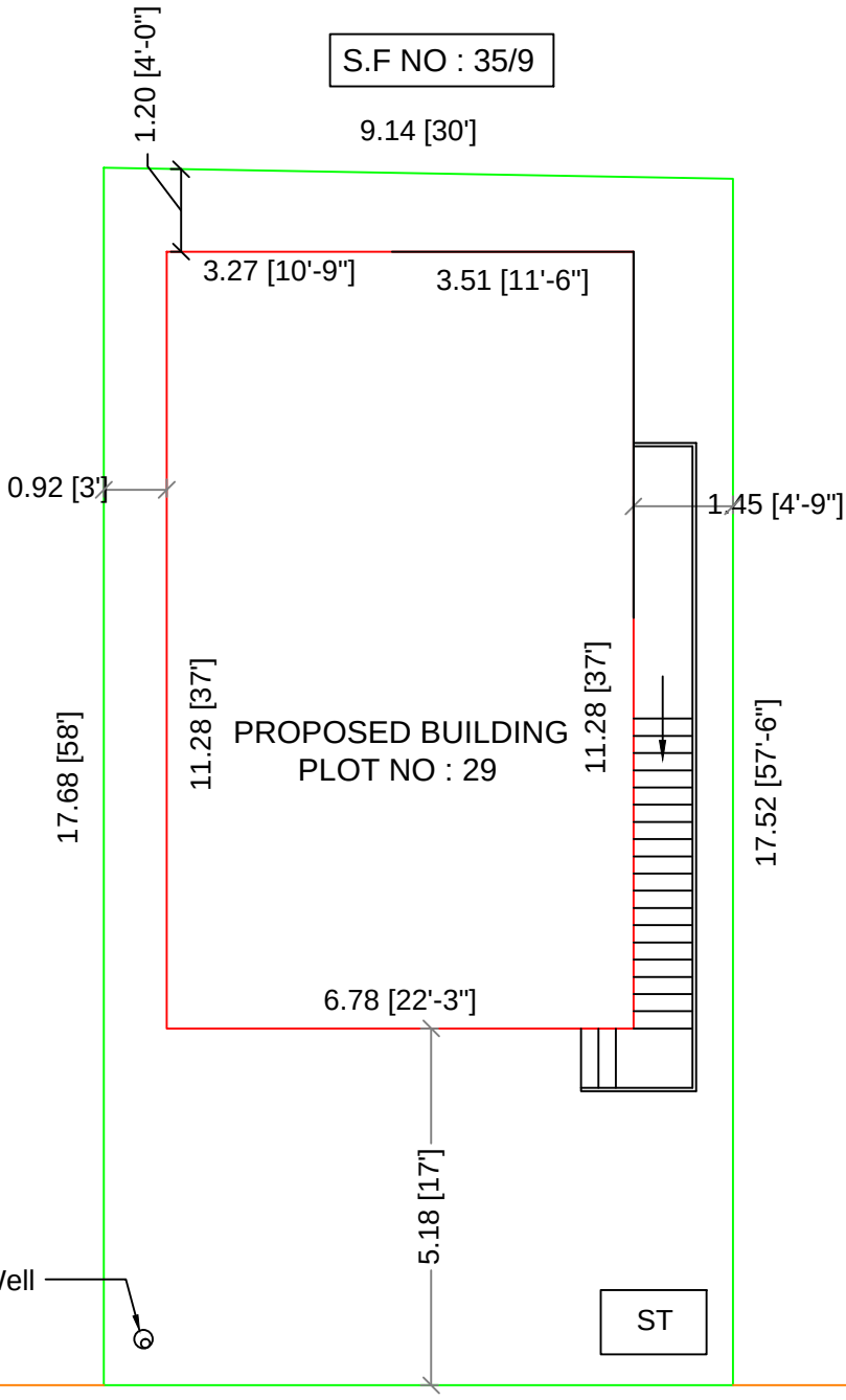
LOCATION PLAN
