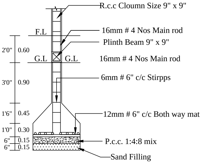
COLUMN DETIAL
