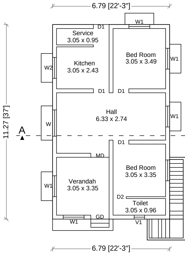
EXG.GROUND FLOOR PLAN
