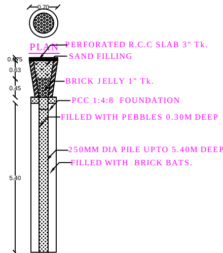
PERCOLATION PIT SECTION OF RAIN WATER
