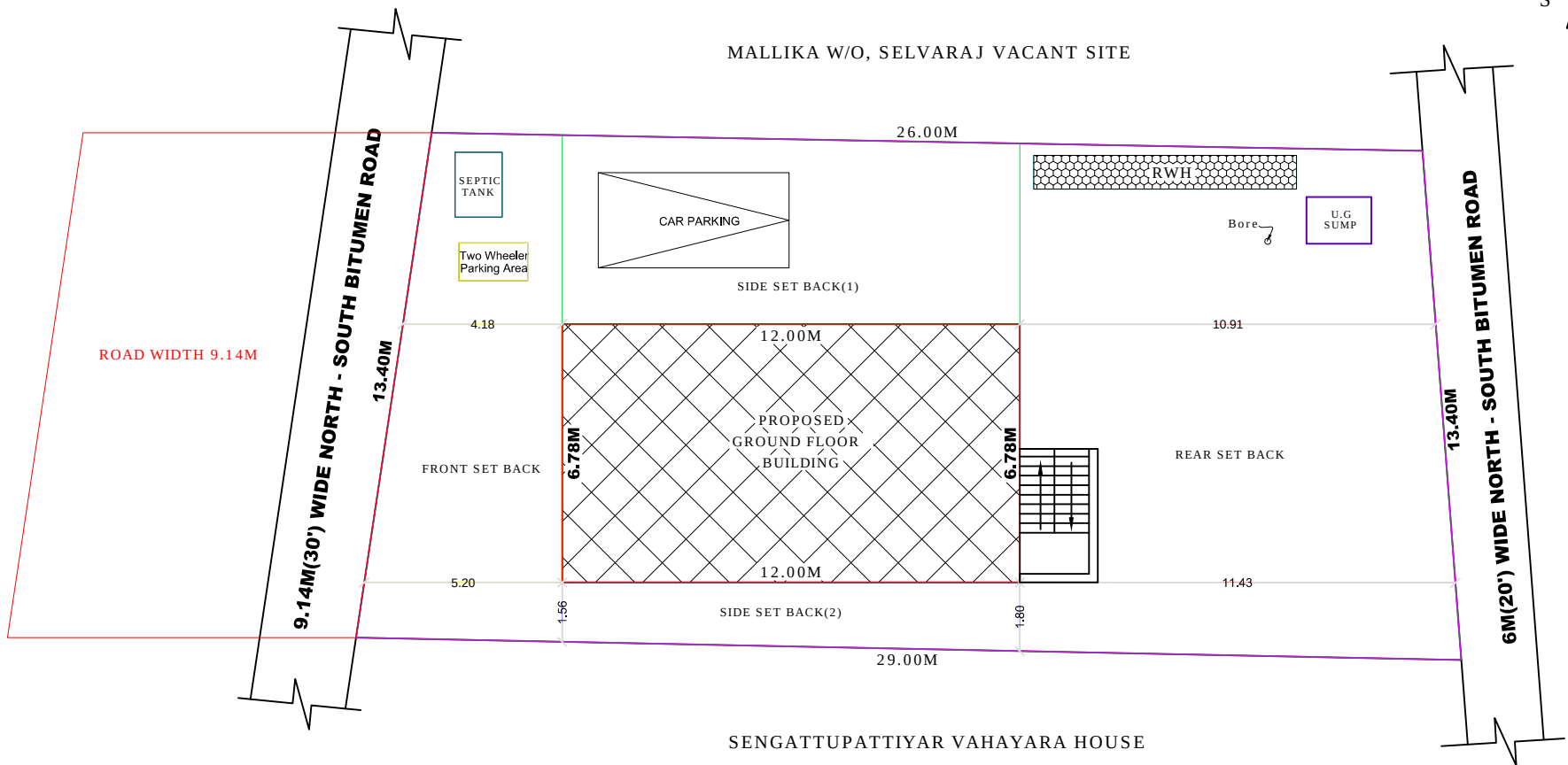
SITE PLAN SCALE = 1:1
