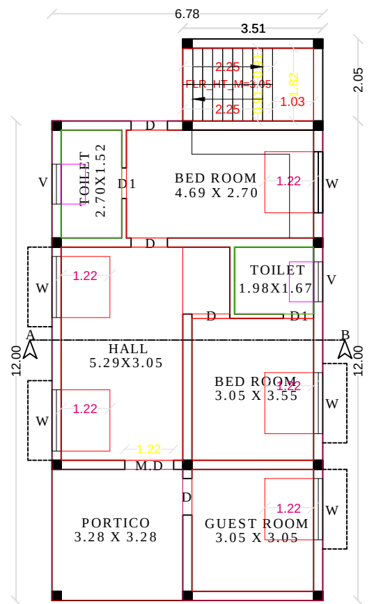
PRO.GROUND FLOOR PLAN (WEST FACING)
