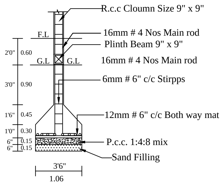
COLUMN DETIAL
