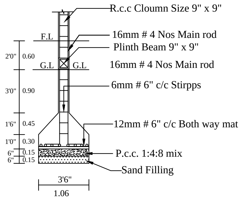
COLUMN DETIAL
