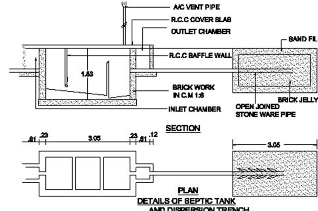
DETAILS OF SEPTIC TANK AND DISPERSION TRENCH
