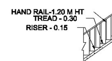
DET - OF STAIRCASE
