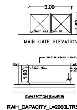
RW_H_CAPACITY_L=2000LTRS
