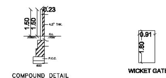
COMPOUND DETAIL
