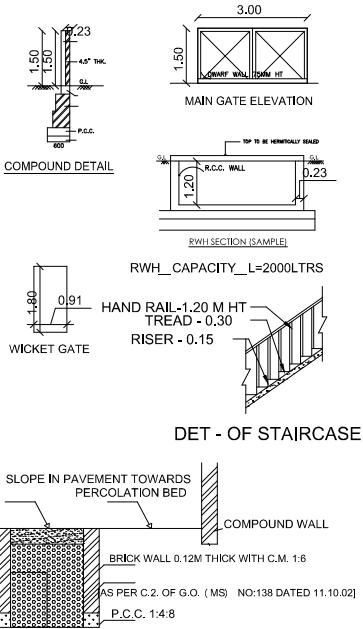
SECTION OF RAIN WATER PERCOLATION BED
