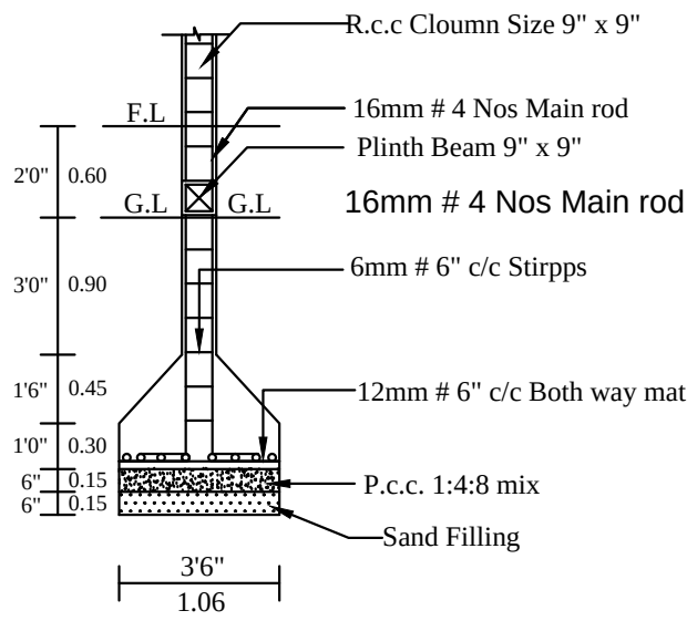
COLUMN DETIAL
