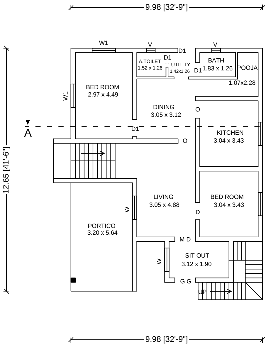
EXG. GROUND FLOOR PLAN
