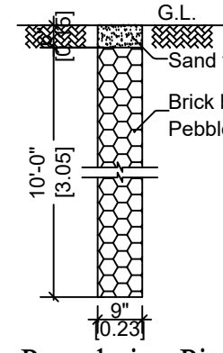
Percolation Pit
