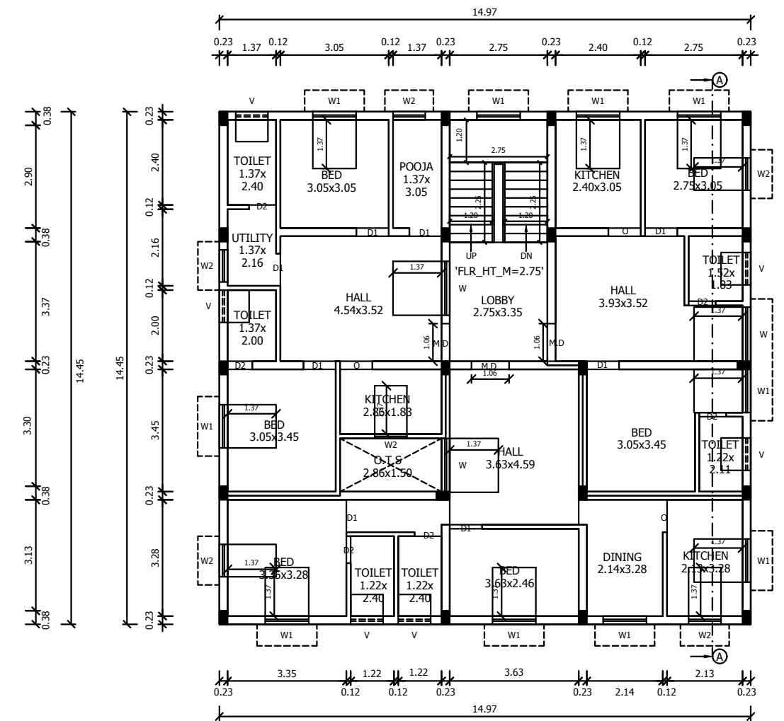
TYPICAL FLOOR PLAN [FIRST & SECOND FLOOR PLAN] TYPICAL_FLOOR_PLAN=1,2
